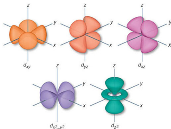
d subshell
