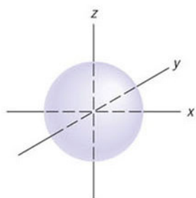
s subshell
