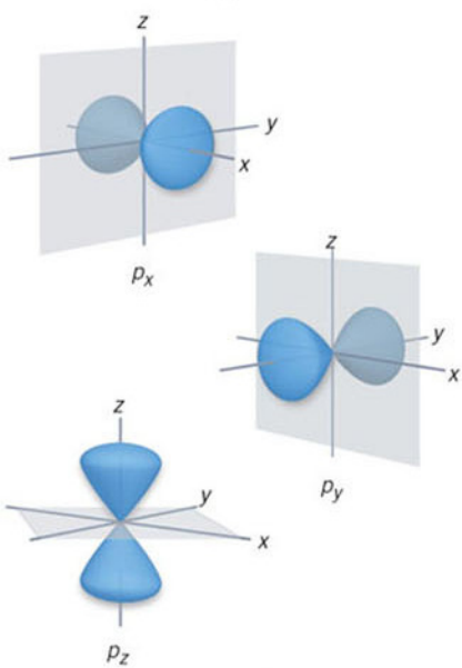
p subshell
